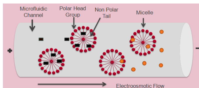
Figure 2.4: Micellar separation of octopamine and dopamine
