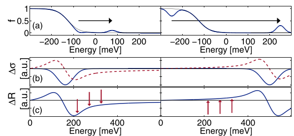
FIG. 4. (a) Nonthermal occupation functions of NbAs, as modeled for pumps of 150 meV (left) and 500 meV (right). The arrow indicates the optical transition made by the pump. Absorption of the lower-energy pump is suppressed by Pauli blocking. The occupation function prior to excitation is shown in the background. (b) The resulting \Delta\sigma_1 (solid) and \Delta\sigma_2 (dashed). (c) \Delta R . The arrows indicate probe energies used.
