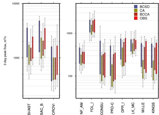
Fig. 7. 3-day peak flow for each streamflow site. Note the vertical axes are different for each of the panels.
